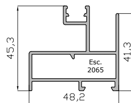
Marco Unicarril Perimetral 15587
