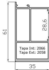
Hoja Central Balconera 17628
