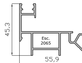
Pluricarril 14647
