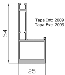
Hoja Central Reducida Balconera 17626
