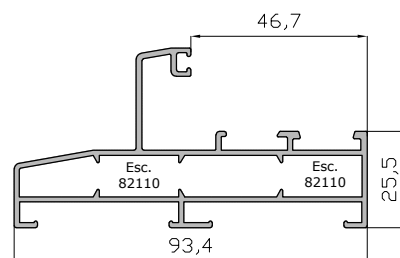
Marco 93.4 mm 5934
