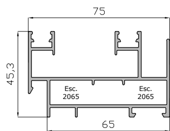
Marco Perimetral 75 mm 14652
