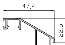
Tapa Monocarril Marco Vertical 15586
