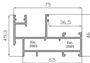
Marco Monocarril Perimetral 15583
