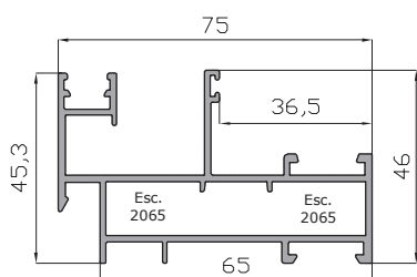
Marco Monocarril Perimetral 15583
