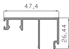
Tapa Monocarril Horizontal 15585
