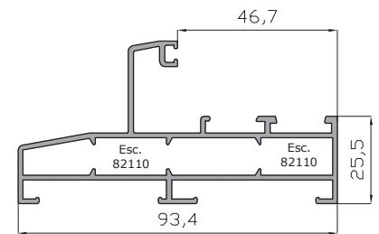
Marco 93.4 mm 5934
