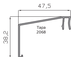
Cumbra 47.5 mm 14655
