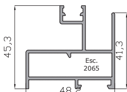
Marco Unicarril Perimetral 15587
