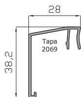
Cumbra 28 mm 14654
