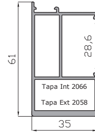
Hoja Central Balconera 17628
