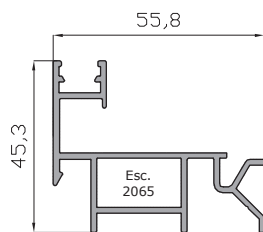
Pluricarril 14647
