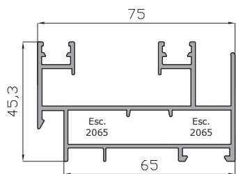
Marco Perimetral 75 mm 14652
