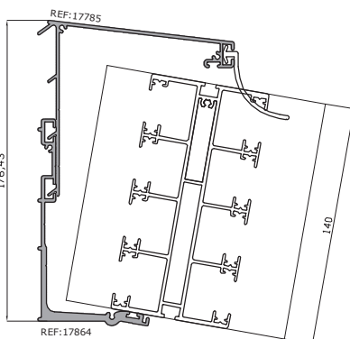
- TECHO 4 CARRILES
