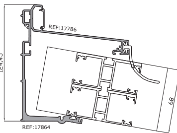
- TECHO 2 CARRILES
