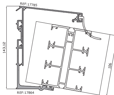
- TECHO 3 CARRILES
