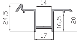
Guia inferior plegable cala 16565
