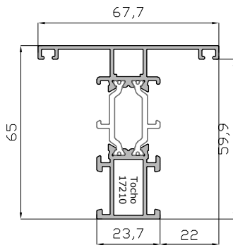
Pilastra Ventana RPT 65 mm 5432
