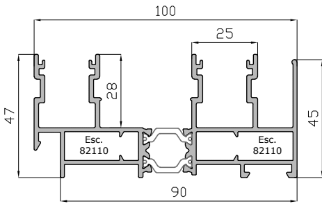
Marco Perimetral 100 mm RPT 15427
