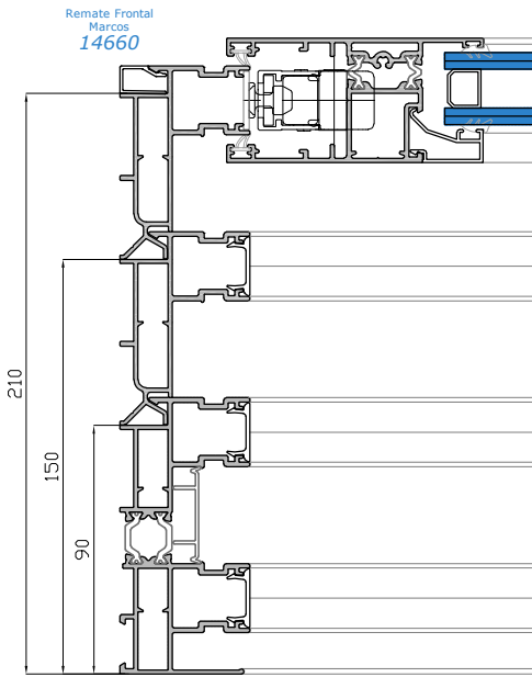
S2 Acople Pluricarril
