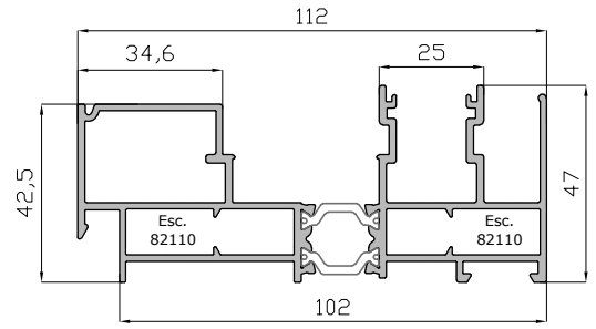
Marco Monocarril Perimetral RPT 15429
