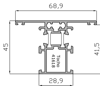
Pilastra Ventana RPT 45 mm 14508
