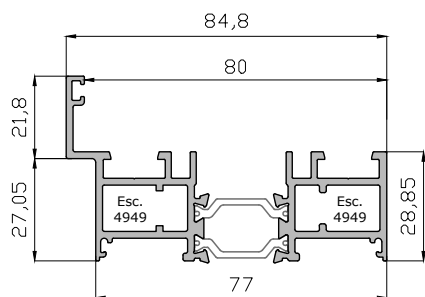
Marco Plegable 12430
