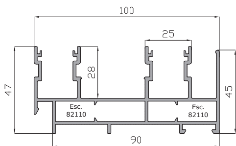
Marco Perimetral 100 mm. 5574
